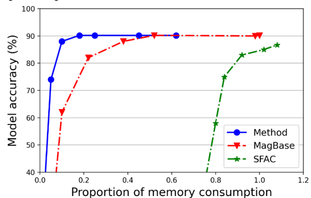
Fig. 1. Compromise between accuracy and memory consumption
