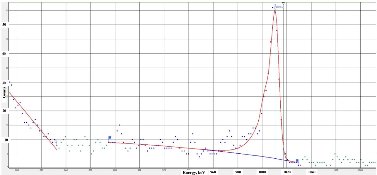
Fig. 7. Gamma-ray spectra processing Source: compiled by the author
