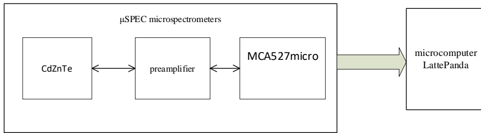
Fig. 4. CZT-spectrometer operation Source: compiled by the author
