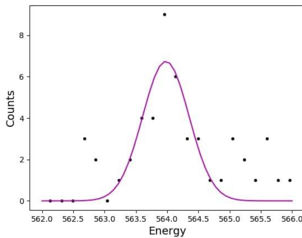
Fig. 8. Gamma-ray spectra processing. Peaks fit Source: compiled by the author
