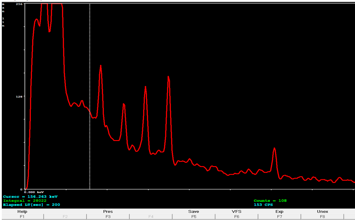
Fig. 2. Gamma-ray spectra 133 Ba Source: compiled by the author
