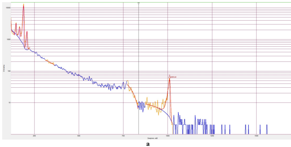
Fig. 5. Gamma-ray spectra processing Source: compiled by the author
