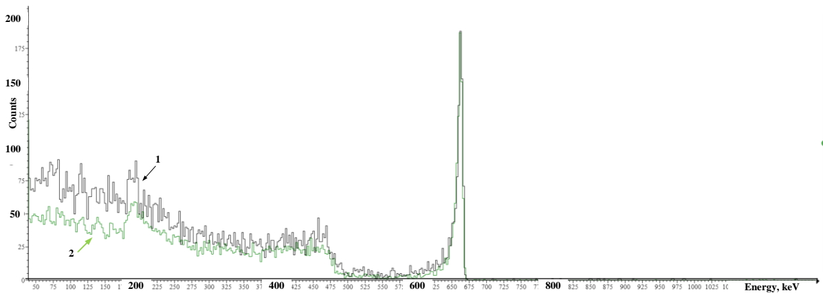
Fig. 9. Gamma-ray spectra processing. Contribution of Compton scattering Source: compiled by the author
