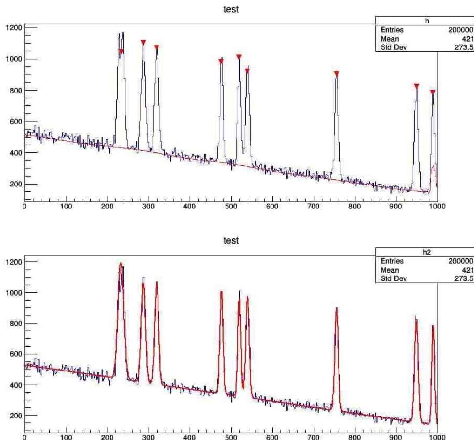
Fig. 3. Gamma-ray spectra processing. Test deconvolution
