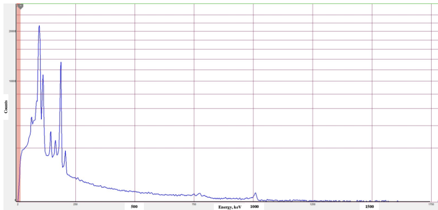
Fig. 5. Gamma-ray spectra processing Source: compiled by the author
