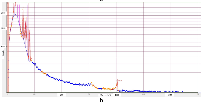
Fig. 6. Gamma-ray spectra processing: a) logarithmic scale; b) quadratic scale Source: compiled by the author
