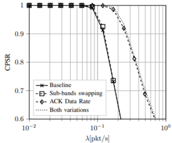
Fig. 6. Impact of improvements on CPSR
