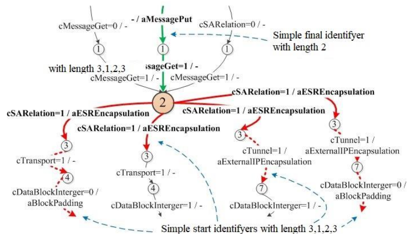
Fig. 2. Identifiers of states/vertexes for behavior diagram
