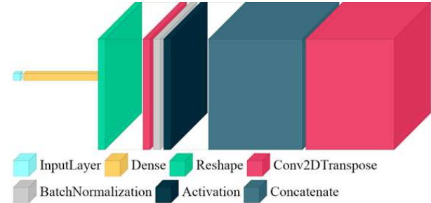
Fig. 10. Architecture of the neural network.
