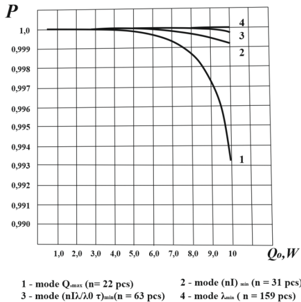
Fig. 9. Relation of single stage TEC failure probability P to thermal load Q_0 for different characteristic current modes at T_0=293\text{K} , T_c=313\text{K} , \Delta T=30\text{K} , l/S=4.5
