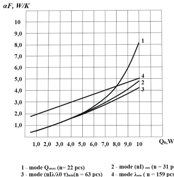
Fig. 10. Dependence of heat dissipation capacity \alpha F of single stage TEC on heat load value Q_0 for different characteristic current modes at T_0=293\text{K} , T_c=313\text{K} , \Delta T=30\text{K} , l/S=4.5
