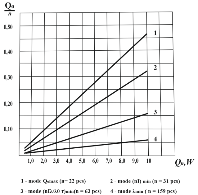
Fig. 5. Dependence of cooling capacity per element \frac{Q_0}{n} of a single stage TEC on the heat load Q_0 for different characteristic current regimes at T_0=293\text{K} , T_c=313\text{K} , \Delta T=30\text{K} , l/S=4.5
