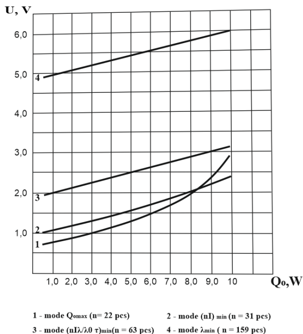
Fig. 4. Dependence of voltage drop U of single stage TEC on heat load value Q_0 for different characteristic current modes at T_0=293\text{K} ,
