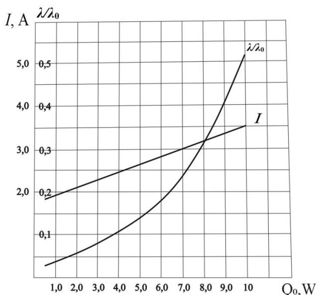
Fig. 11. Dependence of operating current magnitude I , relative failure rate \lambda/\lambda_0 of single stage TEC on heat load magnitude Q_0 in mode (nI\tau\lambda/\lambda_0)_{\min} at T_0=293\text{ K} , T_c=313\text{ K} , \Delta T=30\text{ K} , l/S=4.5
