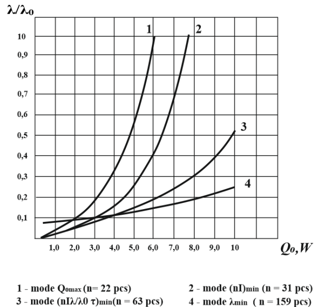
Fig. 8. Dependence of the relative failure rate \lambda/\lambda_0 of a single stage TEC on the thermal load Q_0 for different characteristic current regimes at T_0=293K , T_c=313K , \Delta T=30K , \Delta T=4.5
