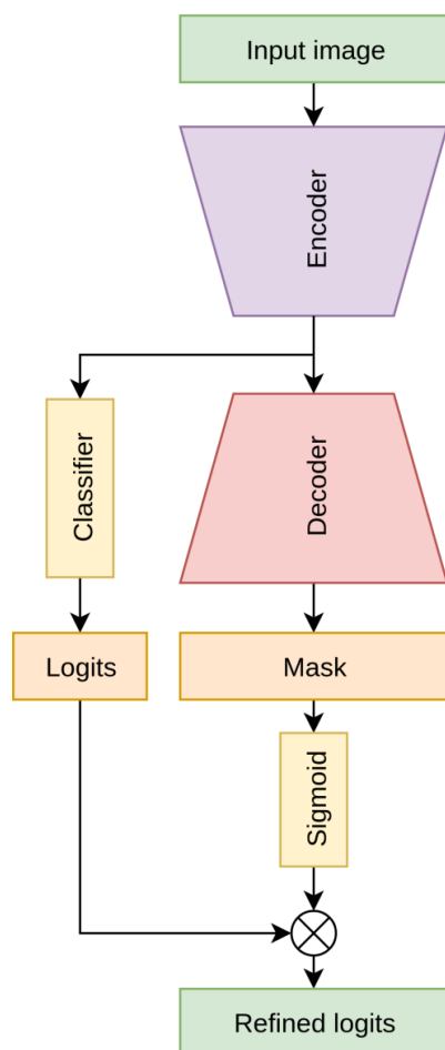
Fig. 6. Network structure during training
