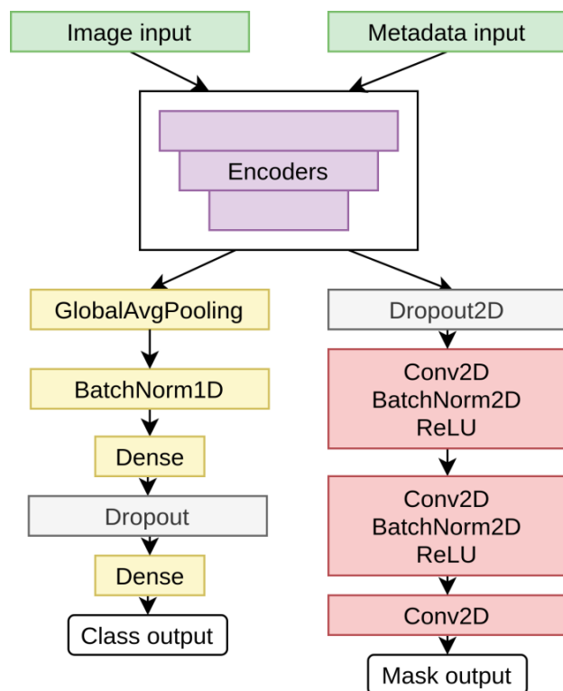
Fig. 7. The detailed architecture of decoders
