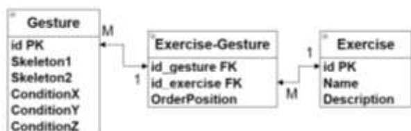
Fig. 9. Relational database model for describing human physical exercises
