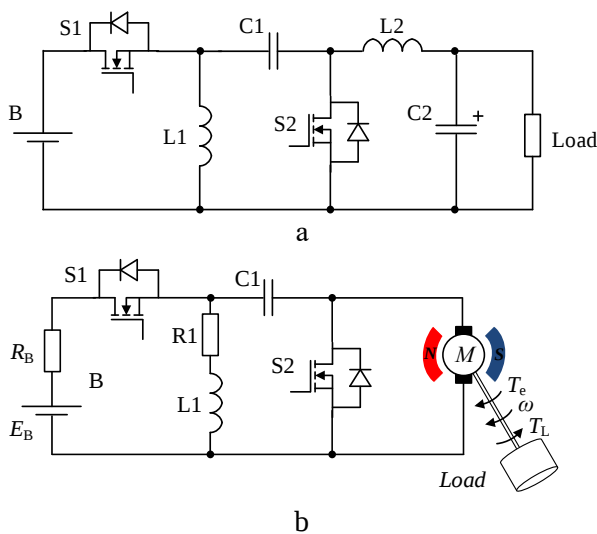
Fig. 1. Scheme of the bidirectional Zeta-SEPIC DC-DC converter (a) and the design scheme of power part of the DC drive system based on it (b) Source: compiled by the authors
