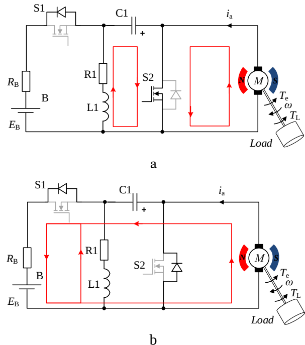
Fig. 3. DC drive in the regenerative braking mode with the SEPIC DC-DC converter during the ON (a) and OFF (b) states of the S_2 switch
