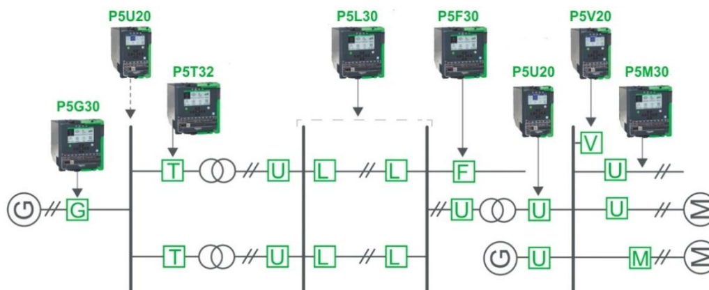
Fig. 2. Overview of Schneider Electric Easergy P5 series devices, where the letters indicate the following protections:
