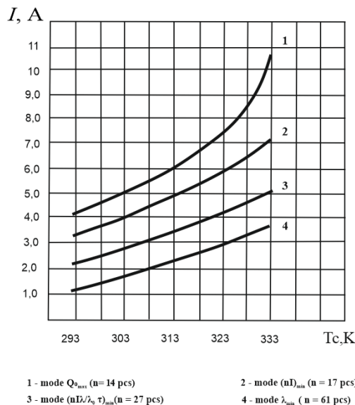
Fig. 2. Dependence of operating current I magnitude on medium temperature T_c for different initial characteristic current operation modes at T_c = 338K at T_0 = 293K; I/S = 4.5;
