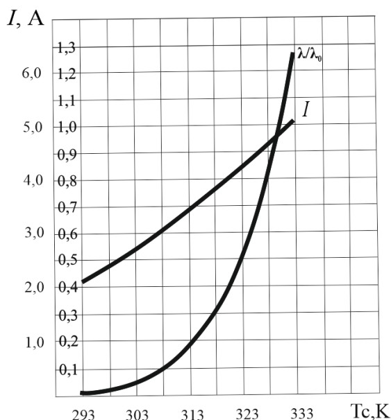
Fig. 11. Dependence of operating current I , relative failure rate \lambda/\lambda_0 on medium
