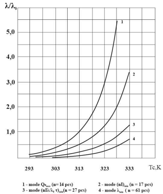
Fig. 9. Relative failure rate \lambda/\lambda_0 dependence on medium temperature T_c for different initial characteristic current modes at T_c = 338\text{K} at T_0 = 293\text{K} ; I/S = 4.5 ; Q_0 = 0.5\text{W} ; t = 10^4\text{h}
