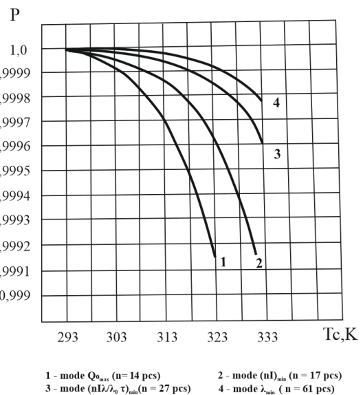
Fig. 10. Failure probability P dependence on medium temperature T_c for different initial characteristic current operation modes at T_c = 338\text{K} at T_0 = 293\text{K} ; I/S = 4.5 ; Q_0 = 0.5\text{W} ;
