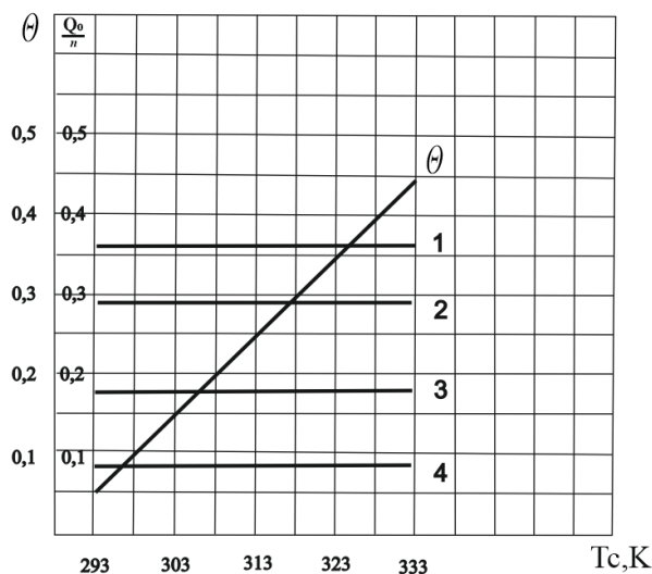
1 - mode Q_{0\max} ( n=14 pcs) 2 - mode (nI)_{\min} ( n=17 pcs) 3 - mode (nI/\lambda_0 \tau)_{\min} ( n=27 pcs) 4 - mode \lambda_{\min} ( n=61 pcs)
