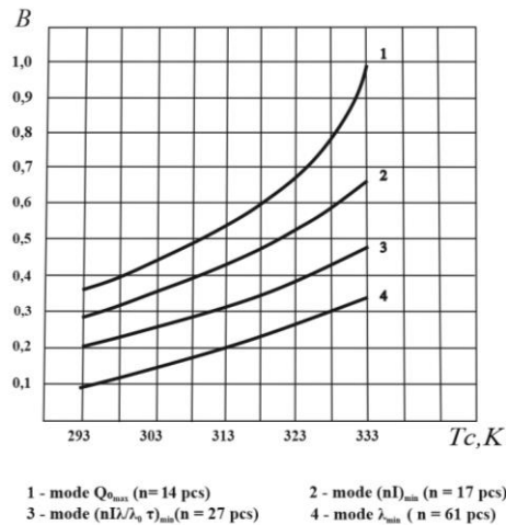
Fig. 1. Relative operating current B vs medium temperature T_c for various initial characteristic current operating conditions at T_c = 338K at
