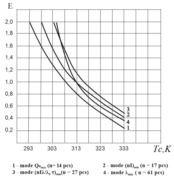
Fig. 3. Dependence of refrigerating factor E on medium temperature T_c for different initial characteristic current operating conditions at T_c = 338K at T_0 = 293K; I/S = 4.5; Q_0 = 0.5W
