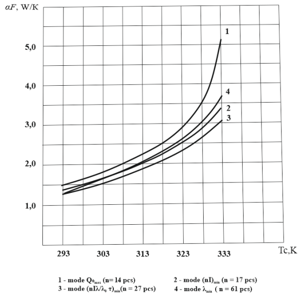
Fig. 8. Dependence of the required heat dissipation capacity \alpha F of the heat sink on the medium temperature T_c for different initial characteristic current operation modes at T_c = 338\text{K} at T_0 = 293\text{K} ; I/S = 4.5 ; Q_0 = 0.5\text{W} ;
