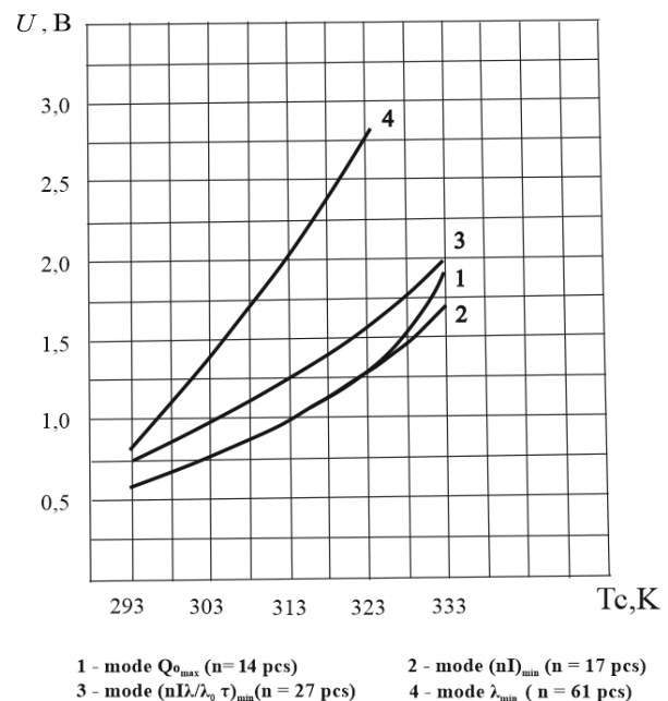
Fig. 4. Dependence of voltage drop U on medium temperature T_c for different initial characteristic current operating modes at T_c = 338K at
