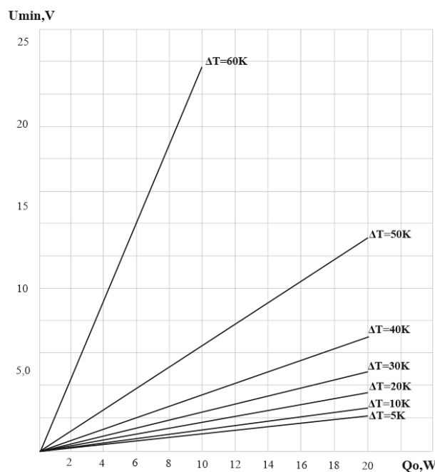
Fig. 4. Dependence of the minimum supply voltage U_{min} of a group of parallel-connected TECs on the heat load Q_0 for different temperature differentials \Delta T at T = 300K, l/S = 4,5
