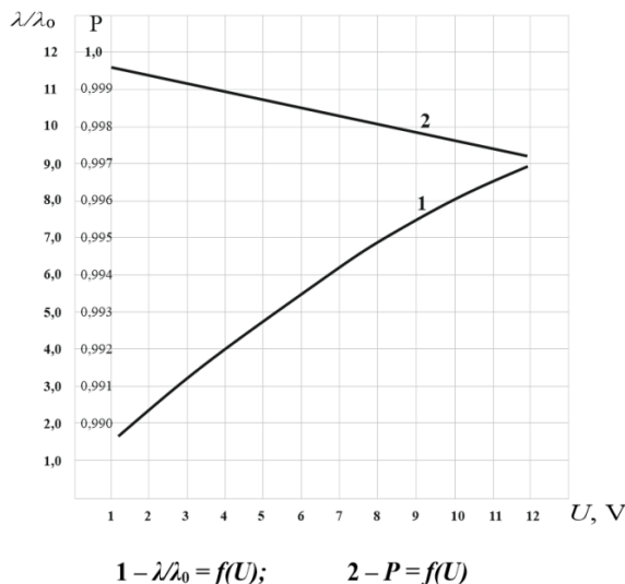
Fig. 17. Dependence of the relative failure rate \lambda/\lambda_0 and the probability P of no-failure operation for the parallel electric connection on the supply voltage U at T = 300K, l/S = 4.5; = 4.5W; \lambda_0 = 3 \cdot 10^{-8} 1/h; t = 10^4 h Source: compiled by the authors
