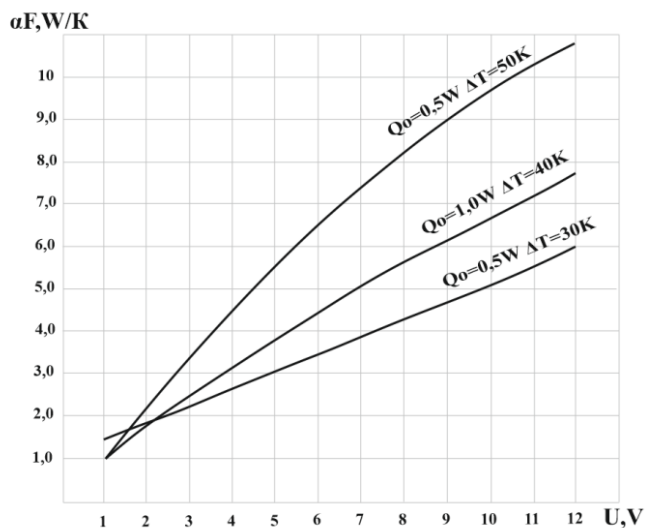
Fig. 11. Dependence of heat dissipation capacity \alpha F of the heatsink from the group with parallel electric connection on supply voltage U for different heat load Q_0 and cooling level T_0 at T = 300\text{K} , l/S = 4.5 Source: compiled by the authors
