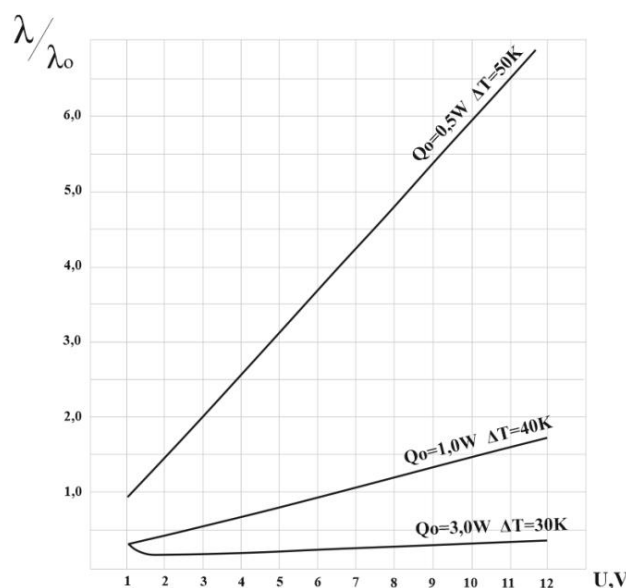
Fig. 13. Dependence of relative failure rate \lambda/\lambda_0 of TECs from the group with parallel electric connection on supply voltage U for different thermal load Q_0 and cooling level T_0 at T = 300\text{K} , l/S = 4.5 Source: compiled by the authors
