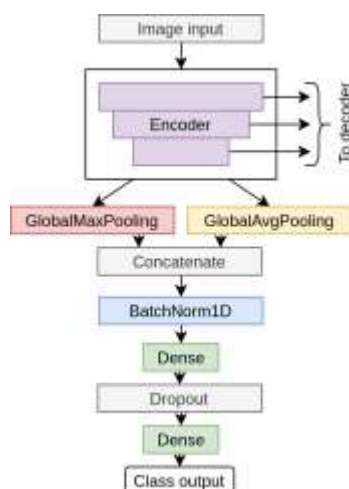
Fig. 5. The architecture of the classifier
