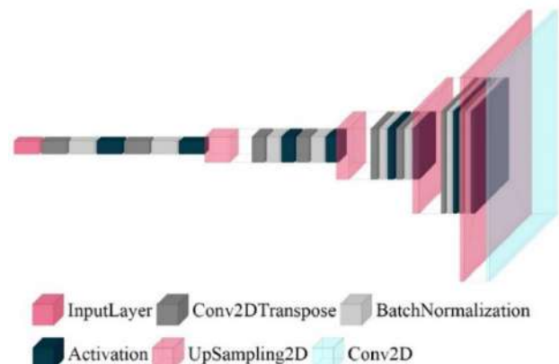
Fig. 9. Architecture of the neural network.
