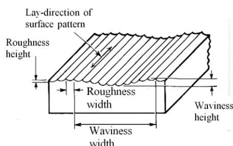
Fig. 2. Surface characteristics (roughness and waviness) excluding surface form deviation
