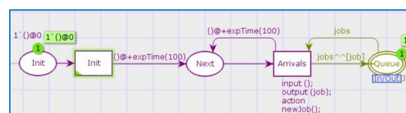
Fig. 7. Web-service request generator model Source: compiled by the authors
