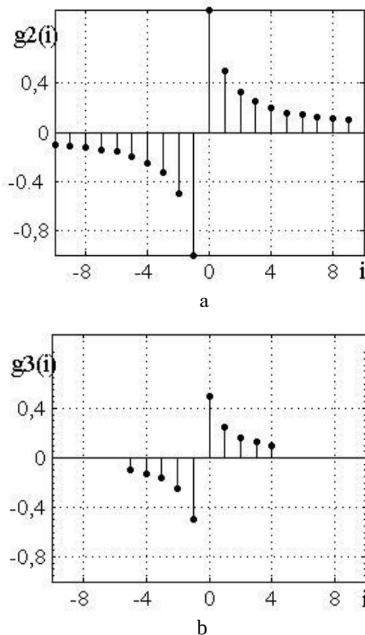
Fig. 2. The impulse response and for WF \Psi_2(i) (a); \Psi_3(i) (b) to evaluate the search direction
