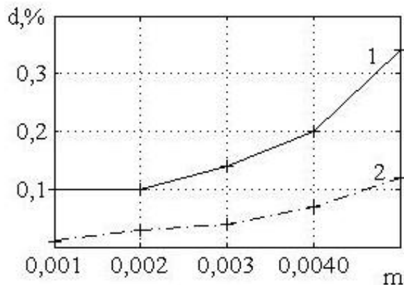
Fig. 3. Relative error ( d ) of asymmetry coefficient ( m ) at determining the extremum:
