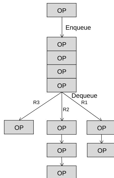
Fig. 5. Operation Queue
