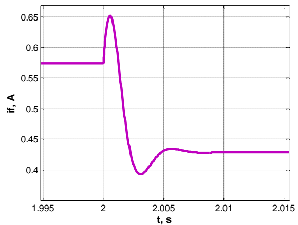
Fig. 21. Excitation current transient process graph in a case of load change Source: compiled by the authors
