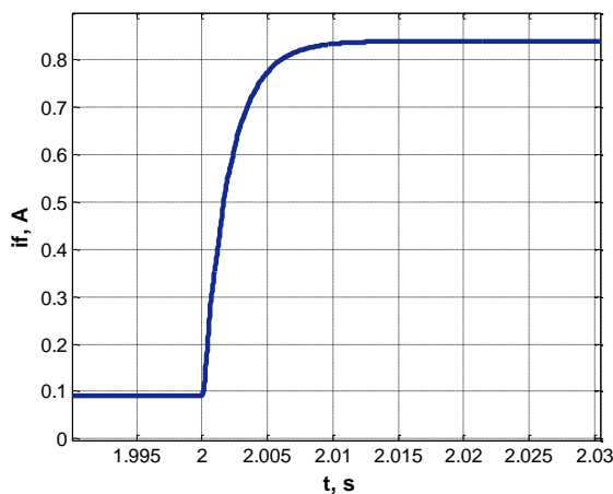
Fig. 19. Field excitation current transient process graph in a case of wind speed change Source: compiled by the authors
