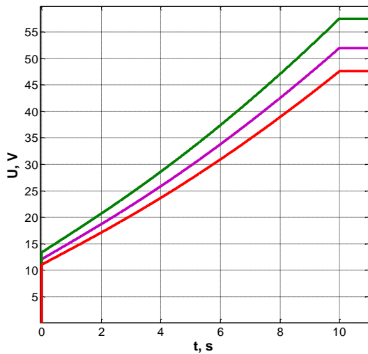
Fig. 18. HESG armature voltage graphs Source: compiled by the authors
