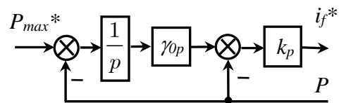
Fig. 10. Maximum HESG power controller diagram of type 101 Source: compiled by the authors
