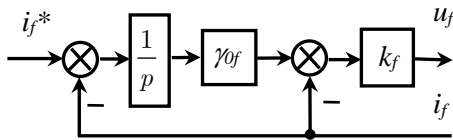
Fig. 8. Field excitation current controller of generator of type 101 Source: compiled by the authors
