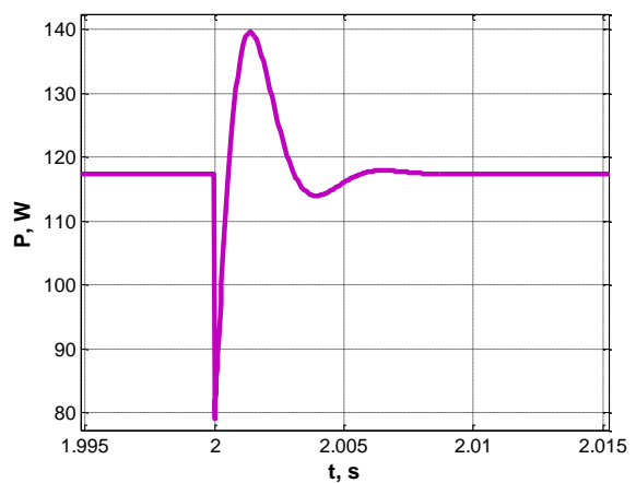
Fig. 22. Maximum output power transient process graph in a case of load change Source: compiled by the authors
