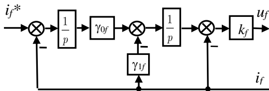
Fig. 9. Field excitation current controller of generator of type 201 Source: compiled by the authors
