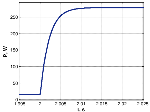
Fig. 20. HESG output electric power transient process graph in a case of wind speed change Source: compiled by the authors
