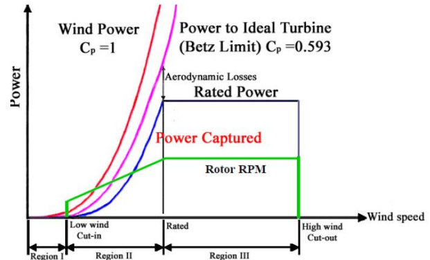
Fig. 2. Turbine output power versus wind speed
