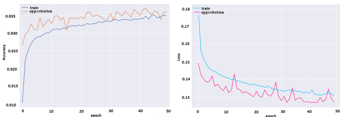
Fig. 6. Accuracy and loss function values during CNN + LSTM deep neural networks approbation for attack detection
